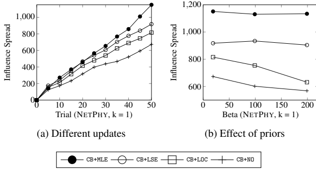
Figure 5: Comparing different updating methods
