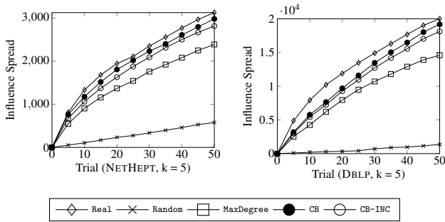
Figure 7: Effectiveness on other datasets
