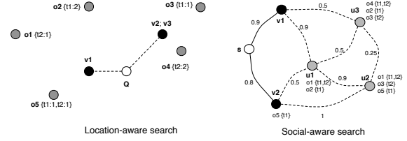
Figure 1: Context-aware search scenarios.
