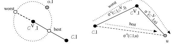
Figure 2: Intuition for start point transpositions.
